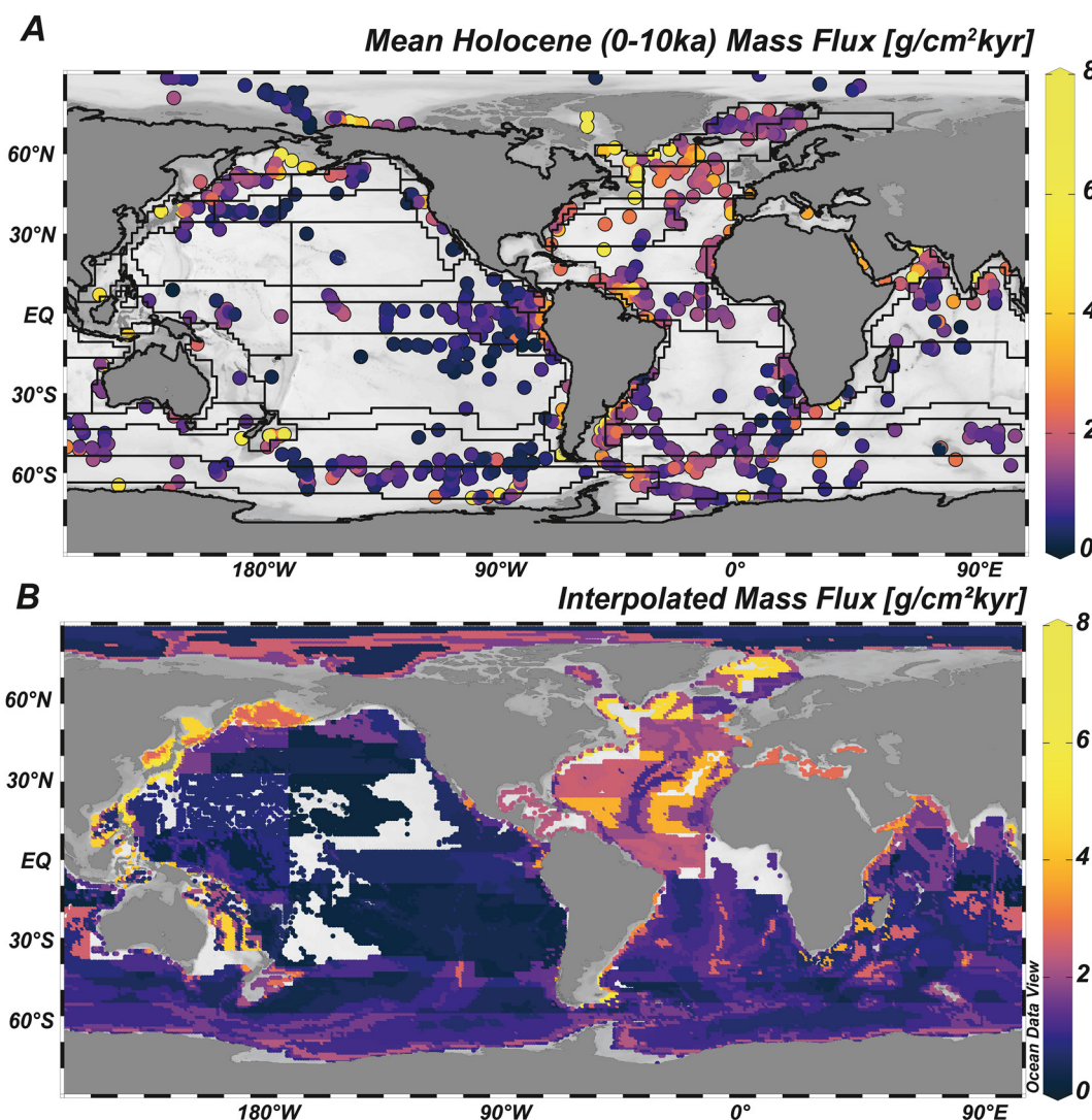
Figure 1. (a) Compiled ^{230}\text{Th} -normalized fluxes from sediment samples of Holocene age (Costa et al., 2020) overlain with the 54 biogeochemical provinces defined by Longhurst (2006) (b) Spatially interpolated ^{230}\text{Th} -normalized fluxes derived by taking the average of available measured fluxes within 145 zones defined by the biogeochemical provinces and water depth. Uncolored (white/gray) zones are shallower than 1 km or zones that do not contain any Th-normalized flux observations.
