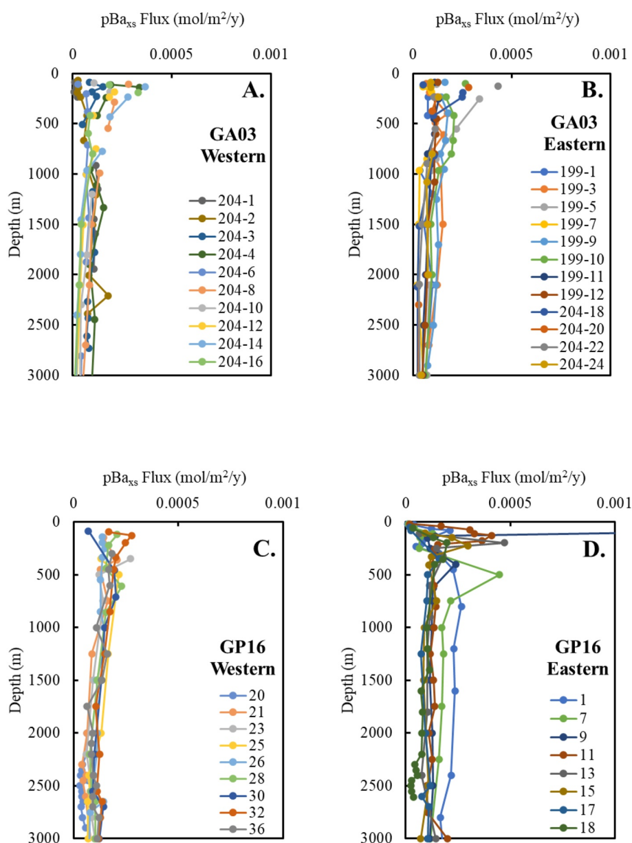
Figure 3. ^{230}\text{Th} -normalized p\text{Ba}_{xs} flux in the water column in the western (a) and eastern (b) basins of GA03. Corresponding ^{230}\text{Th} -normalized \text{Ba}_{xs} flux at stations in the western (c) and eastern (d) basins of GP16 (the maximum flux at station 9, 0.0025 mol m -2 year -1 , is off scale).
